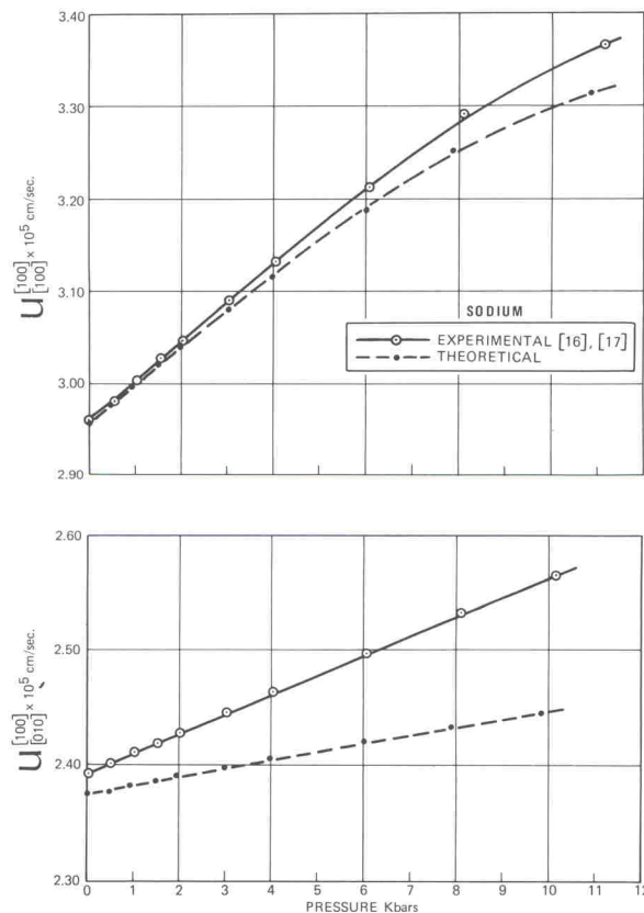
Fig. 1. Variation of U_{[100]/[100]}^{[100]} and U_{[010]/[010]}^{[100]} with pressure for sodium.
